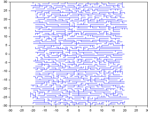
Figure 2: A realization of \mathcal{F}\left(A_{40}^\dagger[200]\right) observed in \mathbb{Z}_{30} .
