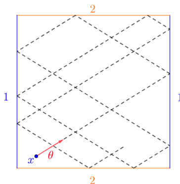
Figure 1: The billiard ball, initially located in x with a momentum \theta , generates the infinite word w = 1211212112\dots
